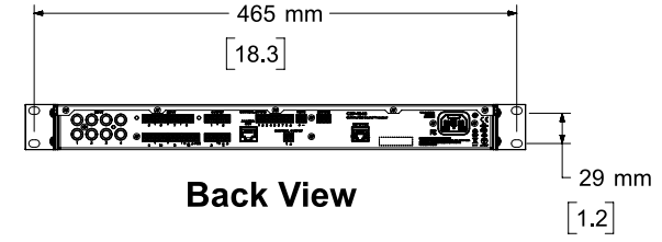
Back View DIMENSIONS APPLY TO BOTH SIDES
