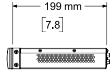
Back View DIMENSIONS APPLY TO BOTH SIDES
