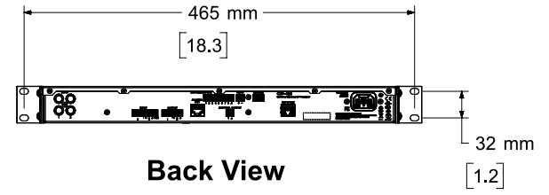
Back View DIMENSIONS APPLY TO BOTH SIDES
