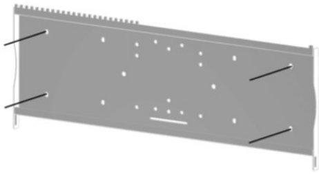
Mounting back plate to the wall
